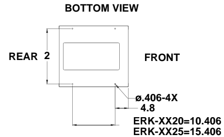
FLOOR MOUNTING LOCATIONS
